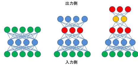
図 3: Stacked-auto-encoder.
